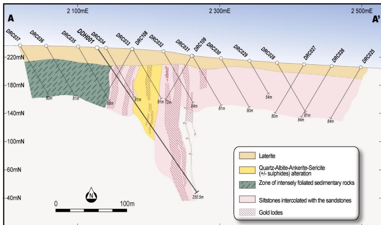
Figure 5: Drilling cross section of the Blaffo Guetto resource area.
